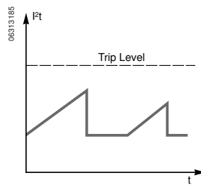
STR Trip Unit without Thermal Memory
