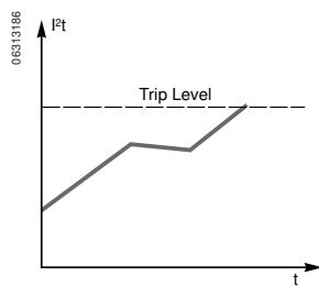
STR Trip Unit with Thermal Memory
