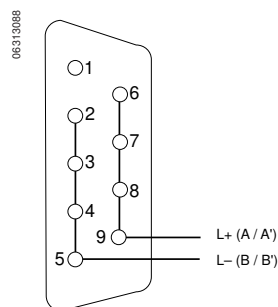
DC150 Concentrator with Polarization and 2-wire Adaptation
