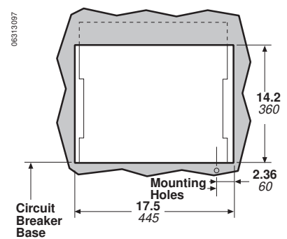
Rear Cutout
