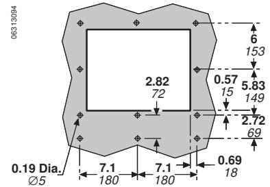
Drilling of the Door
