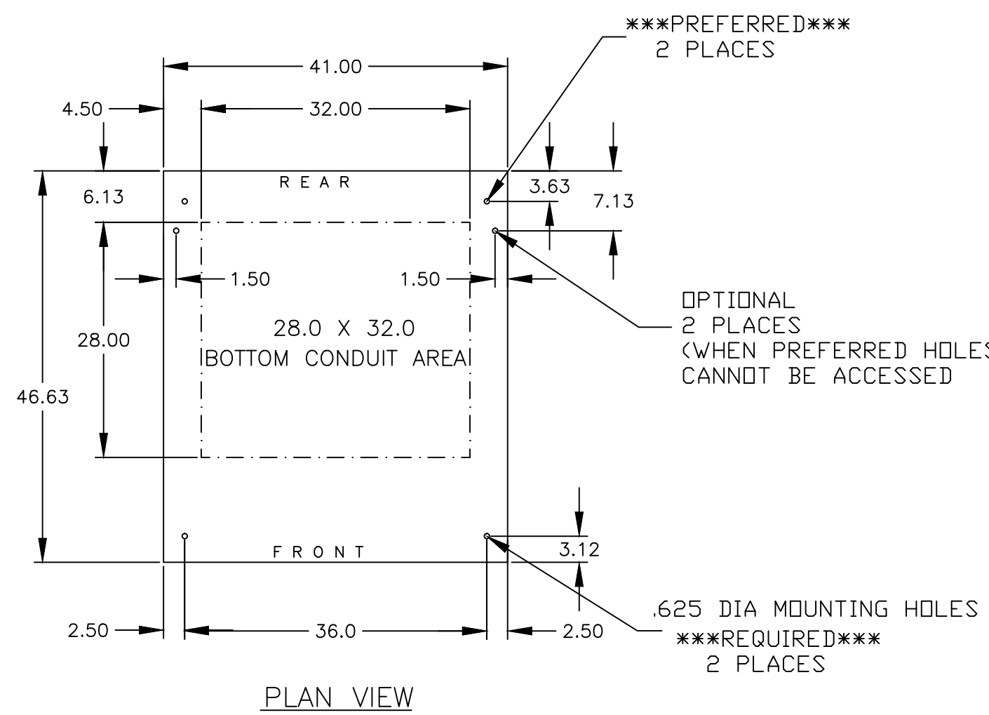
PLAN VIEW
