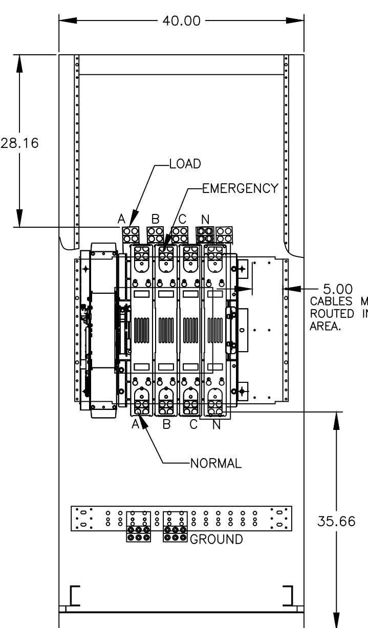
FRONT VIEW WITHOUT COVERS
