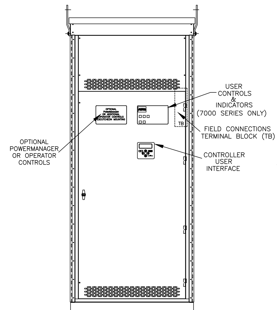
FRONT VIEW WITHOUT EXTERIOR DOOR
