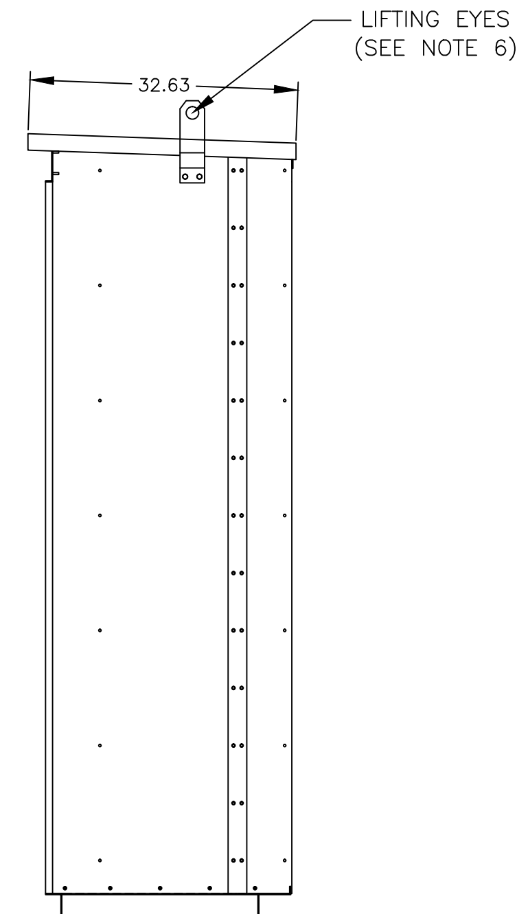
RIGHT SIDE VIEW
