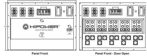
Panel Front
